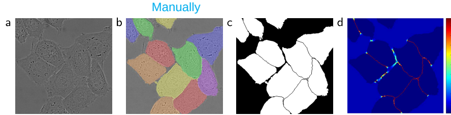
Fig. 3. HeLa cells on glass recorded with DIC (differential interference contrast) microscopy. (a) raw image. (b) overlay with ground truth segmentation. Different colors indicate different instances of the HeLa cells. (c) generated segmentation mask (white: foreground, black: background). (d) map with a pixel-wise loss weight to force the network to learn the border pixels.
